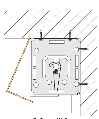
Ceiling or Wall Mounting Endcaps with Optional Fascia
