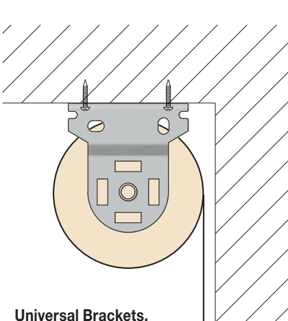
Universal Brackets, Ceiling Mount
