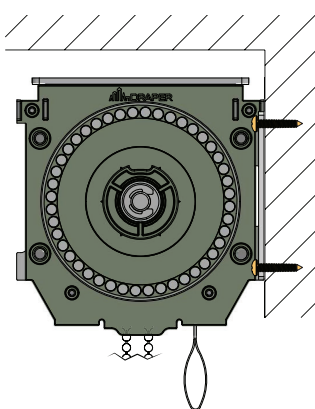
Endcaps Only, Wall Mount
